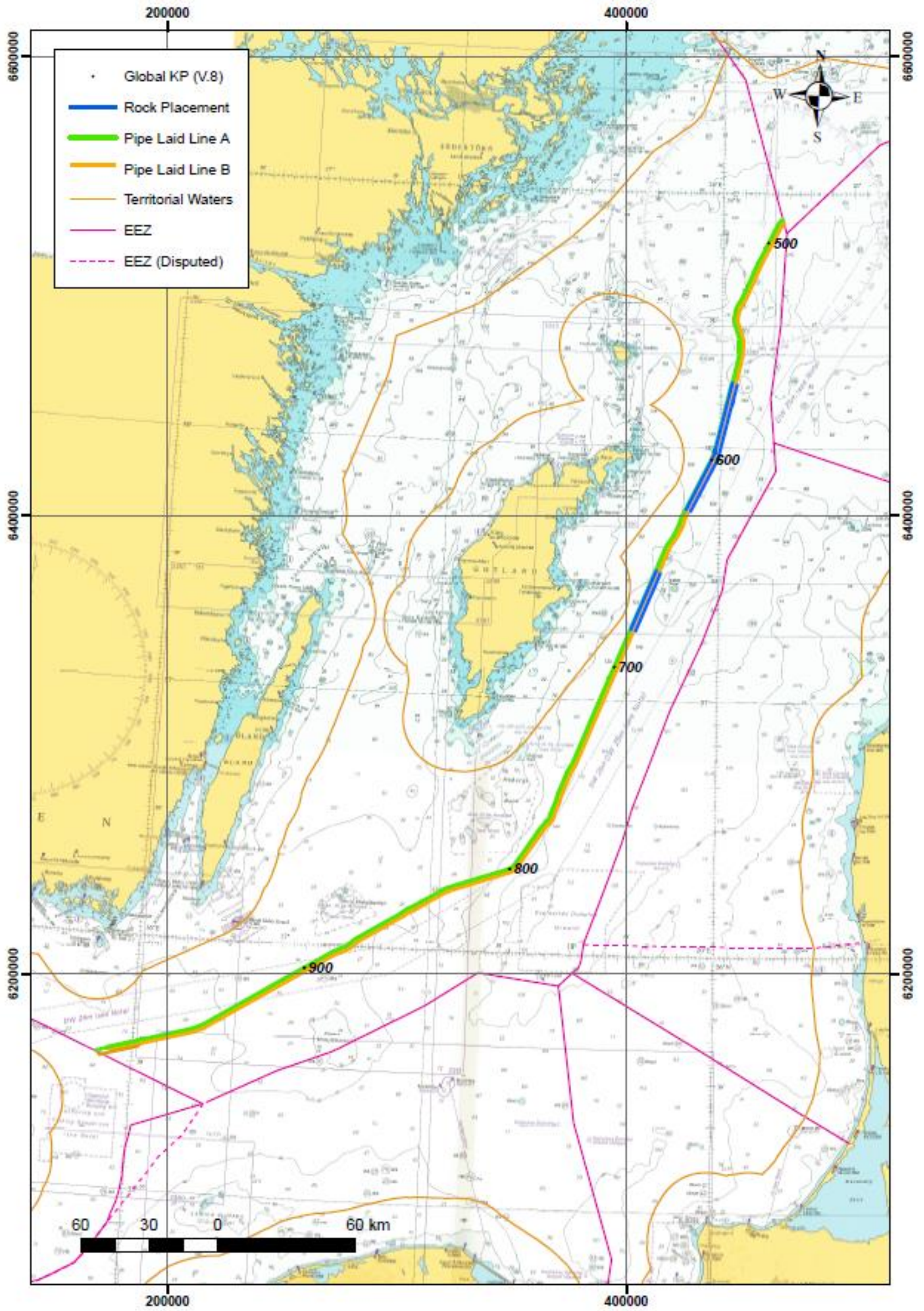
Figure 2: Nord Stream 2 rock placement activities in February in the Swedish EEZ
