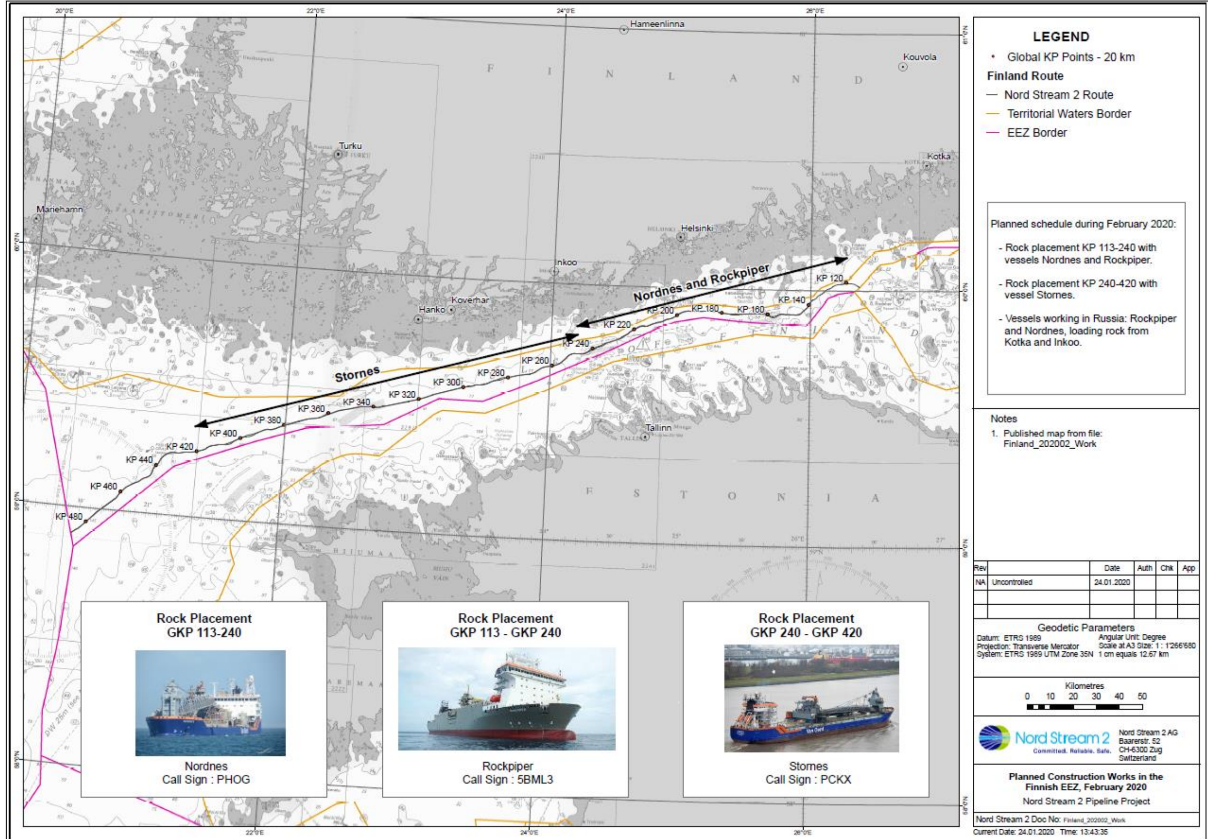
Figure 1: Nord Stream 2 rock placement activities in February in the Finnish EEZ.
